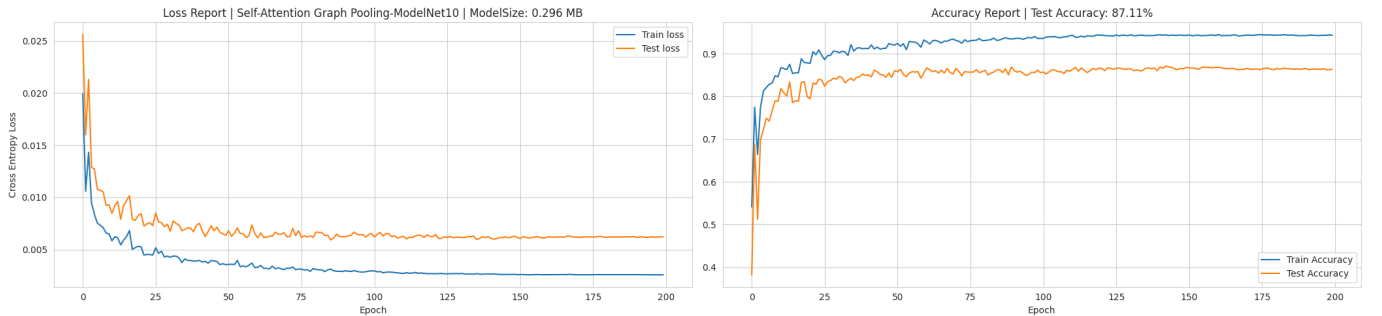
Fig. 4. Training result for original hierarchical SAGPool network On model Net 10.
